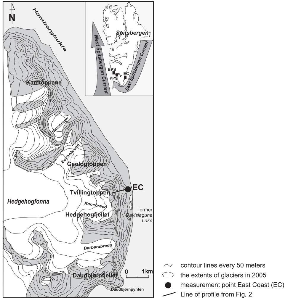
Fig. 1. East Coast measurement point location on Sørkappland. Abbreviations on the Spitsbergen contour map: BPS – Baranowski Polar Station, PPS – Polish Polar Station, EC – East Coast.
