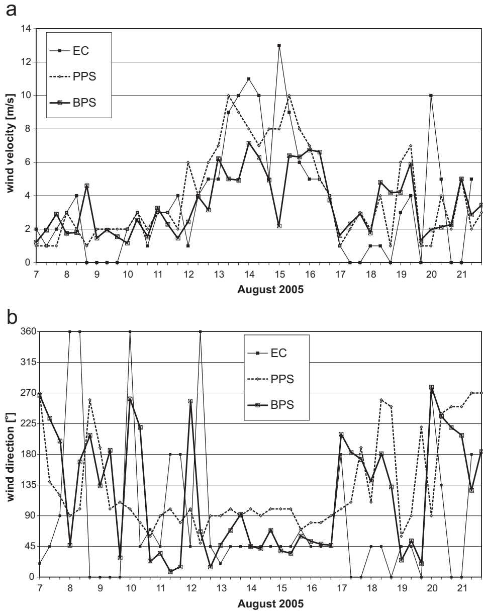
Fig. 7. Wind velocity (a) and direction (b) at East Coast measurement point, Polish Polar Station and Baranowski Polar Station between August 7 and 21, 2005.
