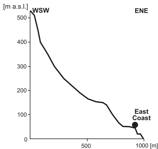
Fig. 2. East Coast measurement point location compared to the relief of the Tvillingtoppen Massif. Refer to Fig. 1 for the position of this profile.
