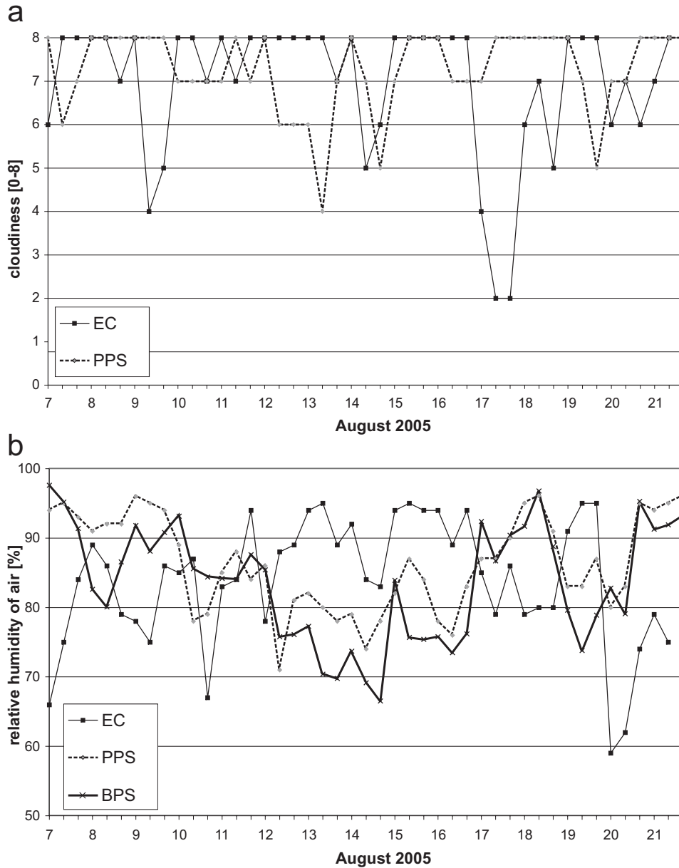
Fig. 5. Cloudiness at East Coast measurement point and Polish Polar Station (a), and relative humidity of air at East Coast measurement point, Polish Polar Station and Baranowski Polar Station (b) between August 7 and 21, 2005.
