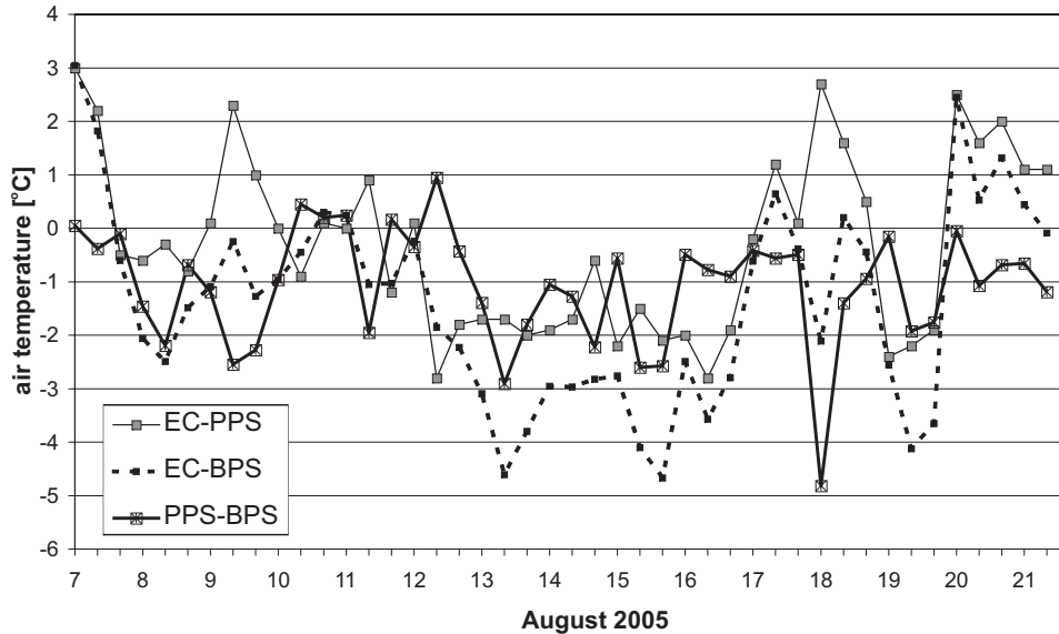
Fig. 8. Air temperature differences between East Coast measurement point and Polish Polar Station and Baranowski Polar Station between August 7 and 21, 2005.
