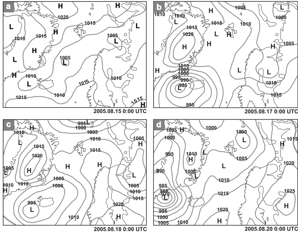
Fig. 6. Pressure field maps for August 15 (a), August 17 (b), August 18 (c) and August 20 (d).
