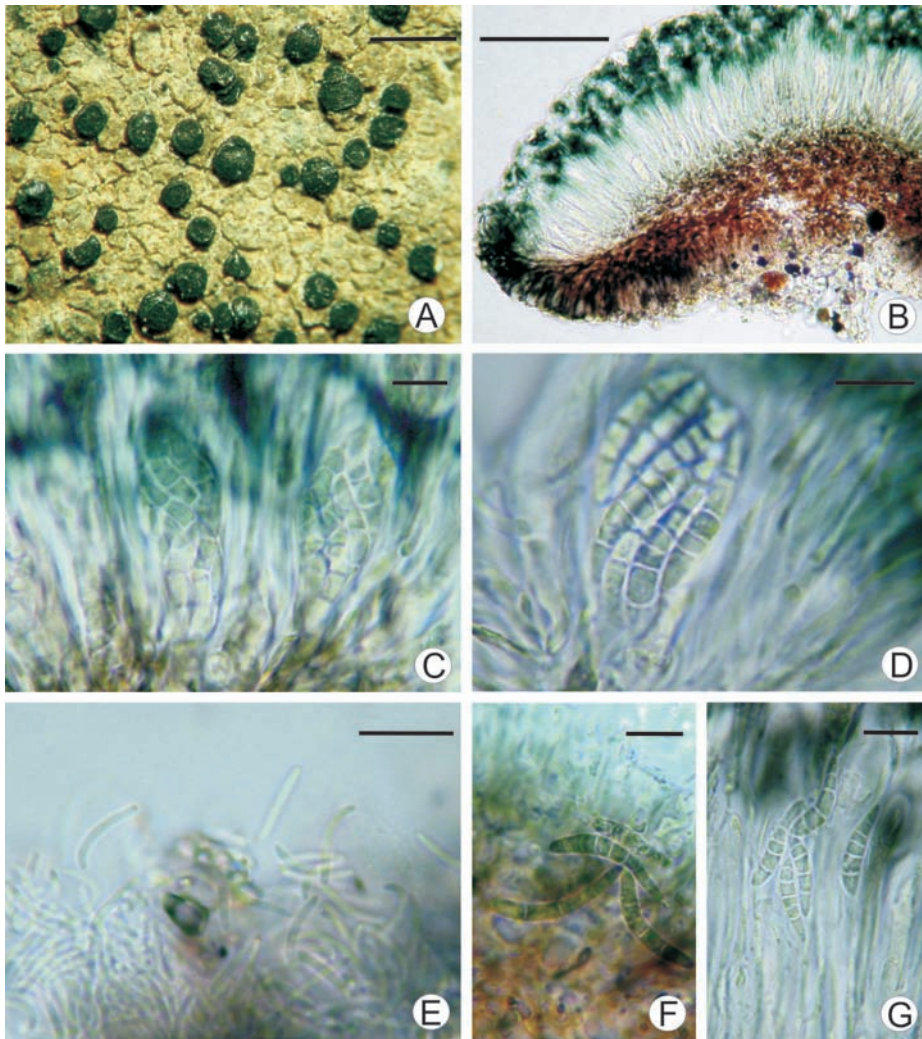
Fig. 2. Bacidia chrysocolla Olech, Czarnota et Llop: (A–E holotype) A – morphology; B – apothecial section; C – coiled asci; D – ascospores; E – filiform conidia; F – ascospores (paratype KRA 8182); G – ascospores (paratype KRA 8183). Scale bars: A – 1 mm; B – 100 \mu m; C–G – 10 \mu m.
