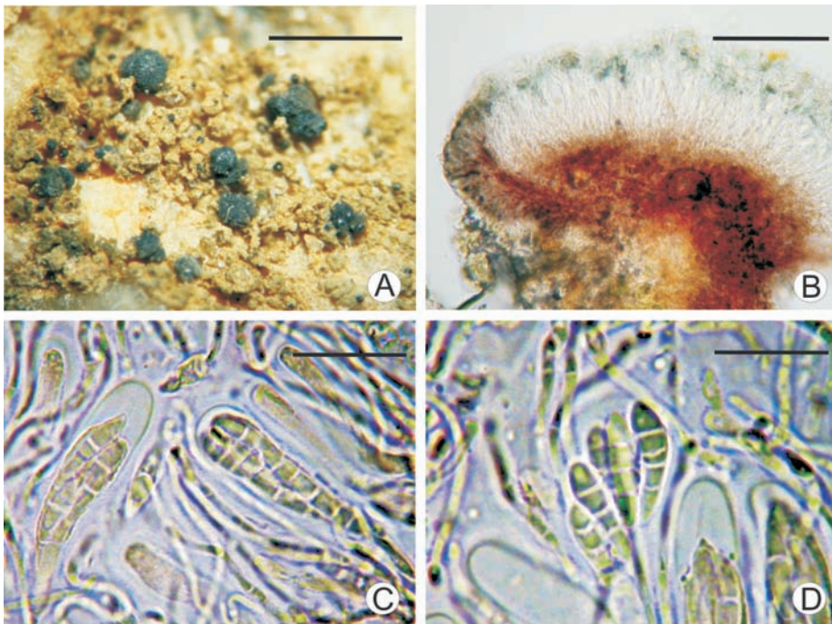
Fig. 1. Bacidia subcoprodes Olech et Czarnota (holotype): A – morphology; B – apothecial section; C – asci with \pm parallelly distributed spores; D – straight and slightly curved ascospores. Scale bars: A – 1 mm; B – 100 \mu m; C and D – 10 \mu m.
